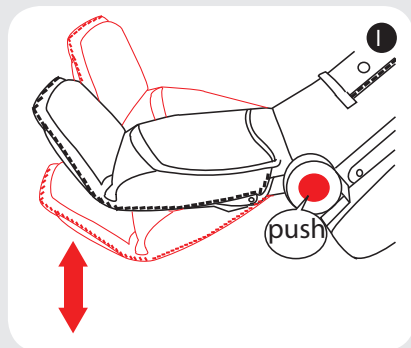
FIGURE I - FOOTREST ADJUSTMENT
